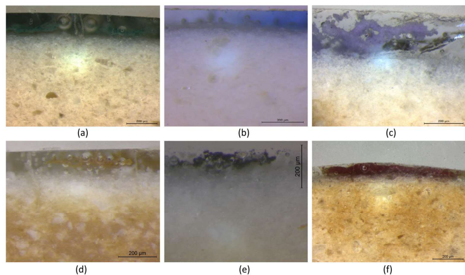
Figure 8. Cross-sections observed under the optical microscope: (a) SAC12 Green; (b) SAC1 intense blue; (c) SAC16 light blue; (d) SAC13 brown; (e) SAC2 black; and (f) MCS9358 pink.
