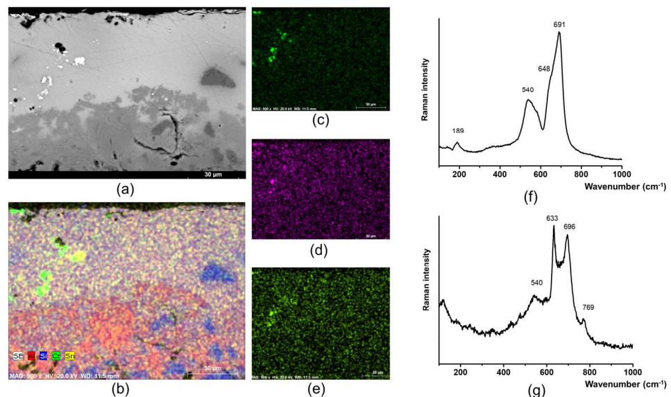
Figure 12. SEM BSE image, elemental maps, and spectral features of the black pigment sample SAC 2. (a) BSE-SEM micrograph of SAC 2; (b) Combination of SE image (a) and elemental map of Al (red), Si (blue), Cr (green), and Sn (yellow); elemental maps of image (a) of (c) Cr, (d) Fe and (e) Co; (f) Raman spectra of chromium-rich and (g) tin-rich particles.
