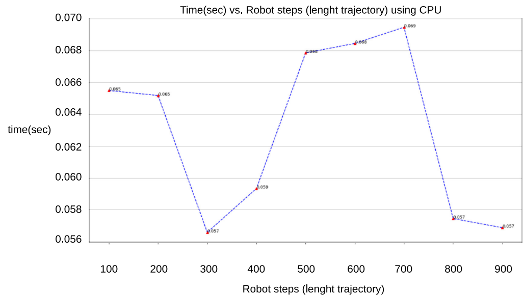
Figure 10. Average time per robot step for varying trajectory lengths with a fixed slide window size of SW = 1203 .
