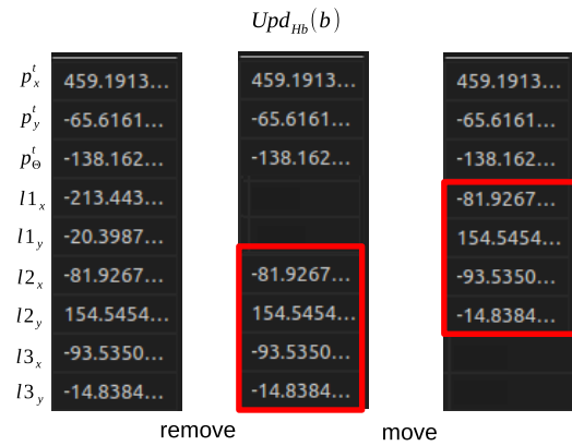
Figure 5. Simple example of updating matrix b where N_{lm} = 1 and k = 3 . The red box highlights the items that are moved during the update.
