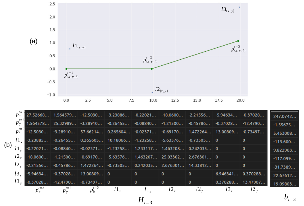
Figure 2. Information matrix H_{t=3} at time step t = 3 , showing the connections between the robot's pose P^{t=3} and the environmental landmarks, while panel (b) shows the information matrix H_{t=3} (left) and the information vector b_{t=3} (right).
