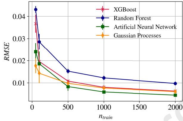
Figure 8: DD laminates: RMSE as a function of the size of the training set, n_{train} , for different algorithms.
