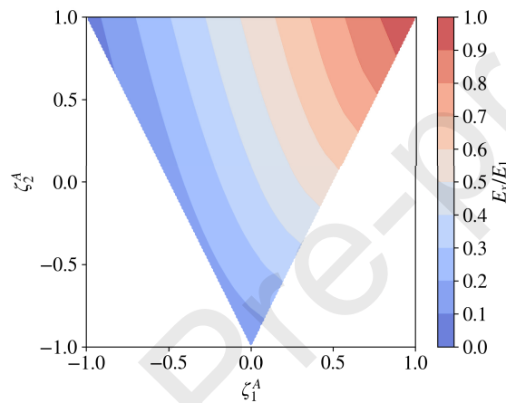
Figure 3: Normalized stiffness as a function of \zeta_{\{1,2\}}^A (valid for 0^\circ/\pm 45^\circ/90^\circ Legacy Quad laminates).
