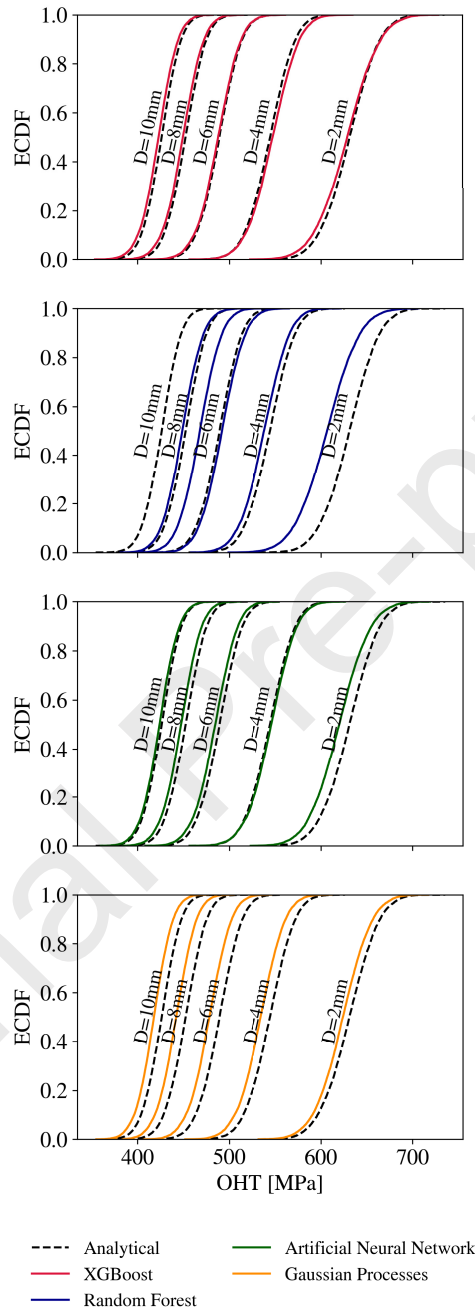
Figure 14: Legacy Quad: ECDF obtained using the analytical model and the trained machine learning models (IM7/8552 [90/0/-45/45] 3s , D=2-10 mm and W=12-60 mm)
