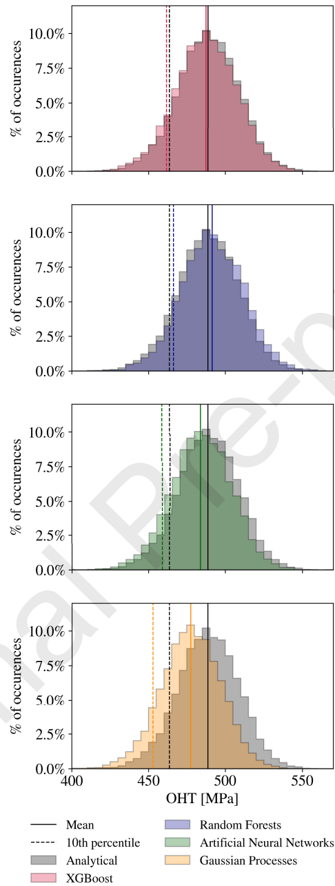
Figure 12: Legacy Quad: distribution of the notched strengths, B-basis (dashed lines) and mean value (full lines) provided by the analytical model and the trained machine learning models (IM7/8552 [90/0/-45/45] 3s , D=6 mm and W=36 mm)
