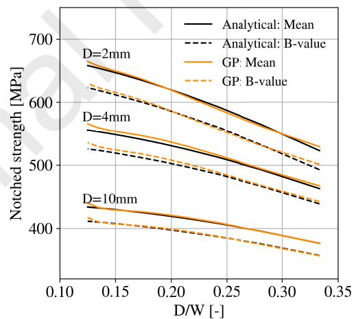
Figure 17: Design chart for diameter-to-width ratio, 1/8 < D/W < 1/3 and hole diameters D = 2, 4, 10 mm for an IM7/8552 [45/-45/20/-20] DD laminate obtained using the analytical framework and the Gaussian Processes model.
