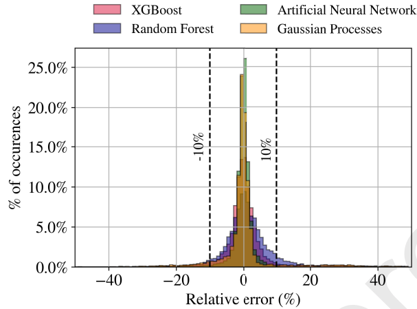
Figure 10: DD laminates: distribution of the relative error for n_{train}=1000 for different algorithms.
