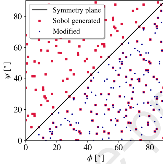
Figure 6: Sobol sampling modification for DD laminates.
