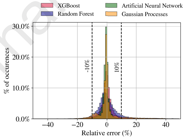
Figure 9: Legacy Quad laminates: distribution of the relative error for n_{train}=1000 for different algorithms.
