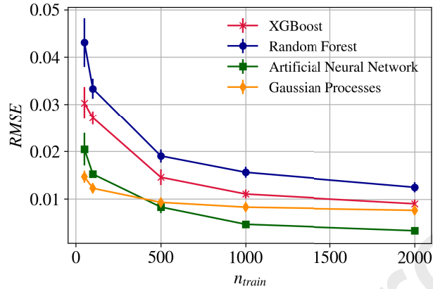
Figure 7: Legacy Quad laminates: RMSE as a function of the size of the training set, n_{train} , for different algorithms.
