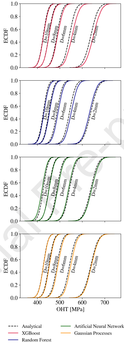
Figure 15: Double-Double: ECDF obtained using the analytical model and the trained machine learning models (IM7/8552 DD [45/-45/20/-20] laminate, D=2-10 mm and W=12-60 mm)
