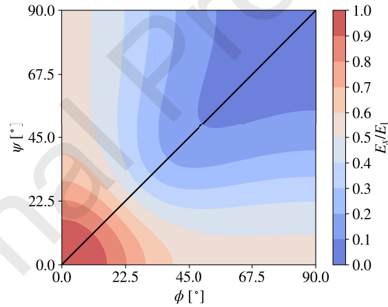
Figure 4: Normalized stiffness of DD laminates as a function of \phi and \psi .
