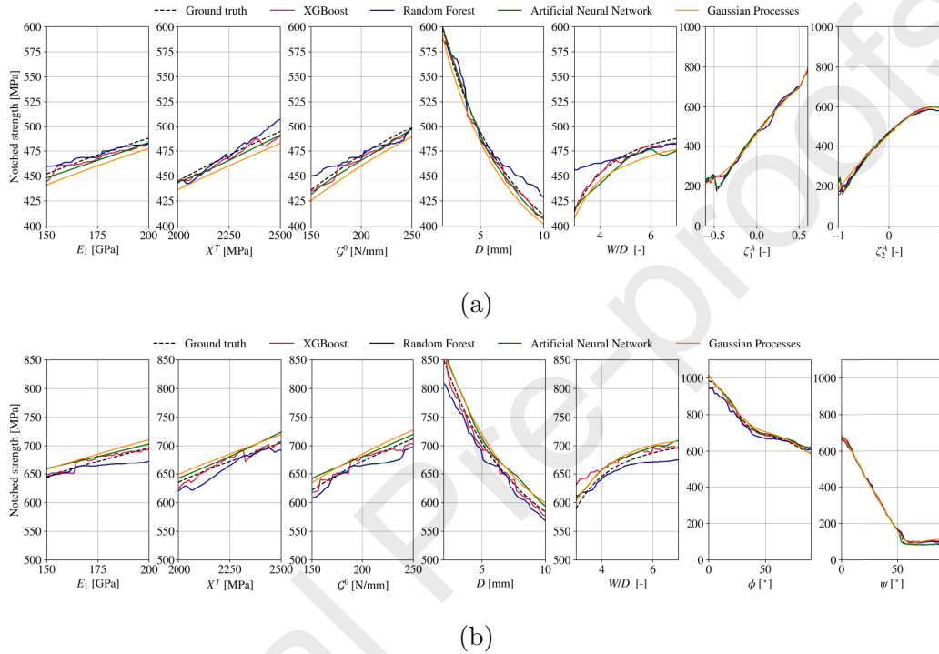
Figure 11: Sensitivity analysis for a) Legacy Quad and b) DD laminates obtained using the four proposed machine learning models ( n_{train}=1000 ). A single parameter is varied ranging from its allowed minimum and maximum, while the remaining are kept constant at E_1=175 GPa, X^T=2250 MPa, G^0=200 N/mm, D=6 mm, W/D=5 , \zeta_1^A=0 , \zeta_1^A=0 (for QUAD laminates) and \phi=60^\circ , \psi=0^\circ (for DD laminates). Note that in the last subfigure, a plateau appears for \psi value above 60^\circ . As the value of \phi is fixed at 60^\circ , these laminates are very "soft", and present a matrix dominated failure for which the current analytical model predicts very similar behaviours.
