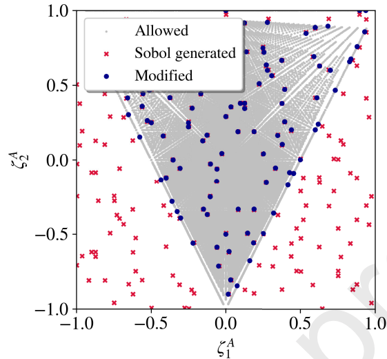
Figure 5: Sobol sampling modification for Legacy Quad laminates.
