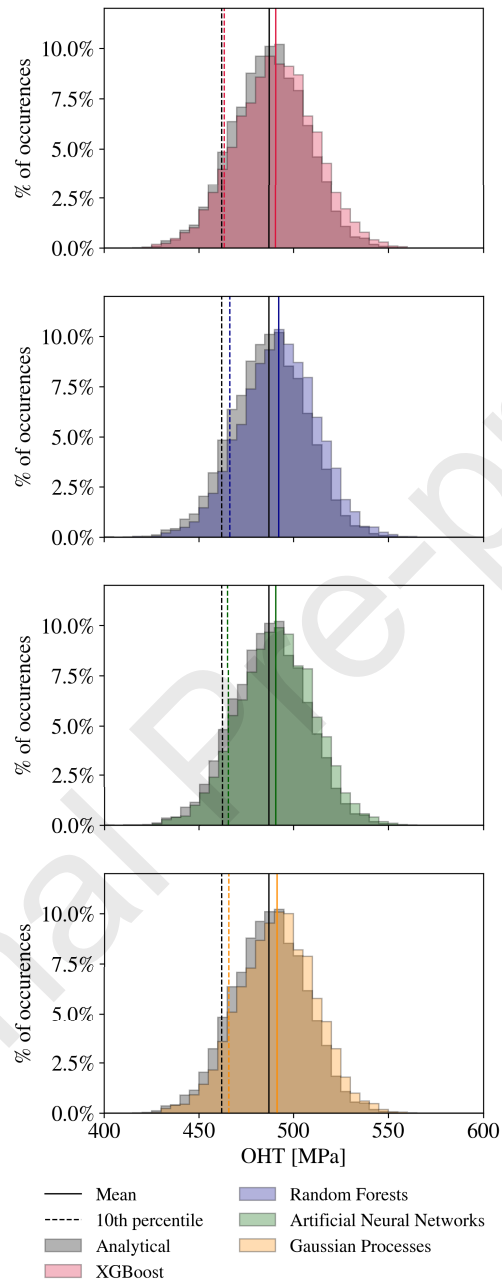
Figure 13: Double-Double: distribution of the notched strengths, B-basis (dashed lines) and mean value (full lines) provided by the analytical model and the trained machine learning models (IM7/8552 DD [45/-45/20/-20] laminate, D=6 mm and W=36 mm)
