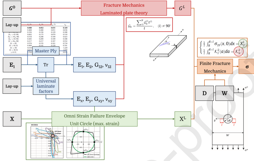
Figure 2: Schematic representation of the proposed combined framework to predict size effects from the minimum number of properties determined at the ply level.
