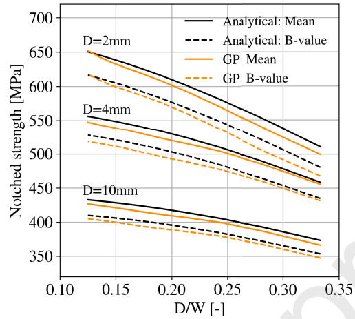
Figure 16: Design chart for diameter-to-width ratio, 1/8 < D/W < 1/3 and hole diameters D = 2, 4, 10 mm for an IM7/8552 [90/0/-45/45]_{3s} Legacy Quad laminate obtained using the analytical framework and the Gaussian Processes model.
