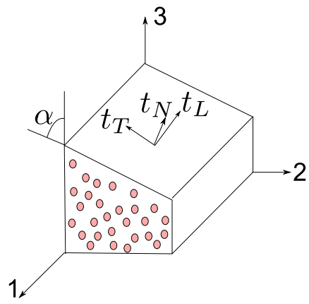
Fig. 1. Components of traction on the fracture plane
