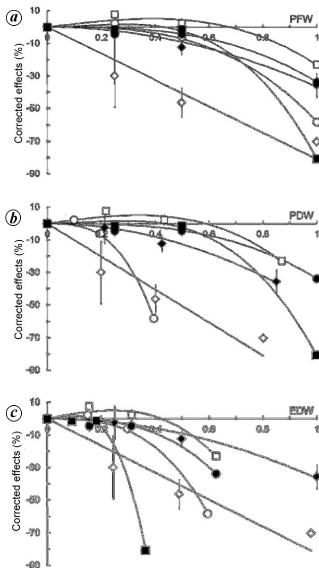
Figure 2. Expected and observed effects of extracts corrected for pH and osmotic pressure on germination of L. sativa cv. 'Rainha de Maio' (means \pm SE). Extract concentrations are expressed as (a) PFW, (b) PDW and (c) EDW. Concentrations were normed so that the highest value was unity. Open circles, Foeniculum vulgare ; filled circles, Cistus ladanifer ; open squares, Cistus monspeliensis ; filled squares, Calicotome villosa ; open diamonds, Lavandula stoechas and filled diamonds, Daphne gnidium .
