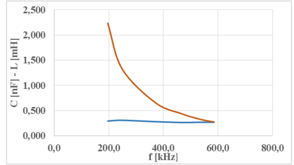
Fig. 3. Tuning of the transmitter circuit.
