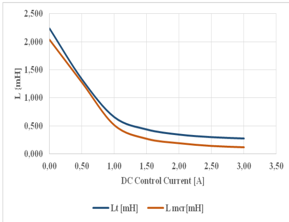
Fig. 2. Inductance variation with the DC control current.
