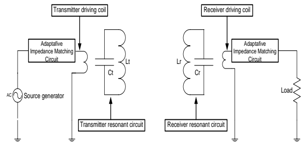
Fig. 1. WPT via strongly coupled magnetic resonance.
