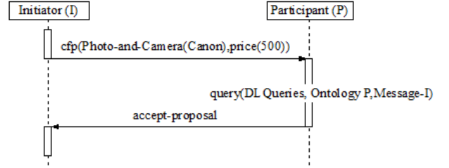
Figure 2: AUML negotiation interaction.
