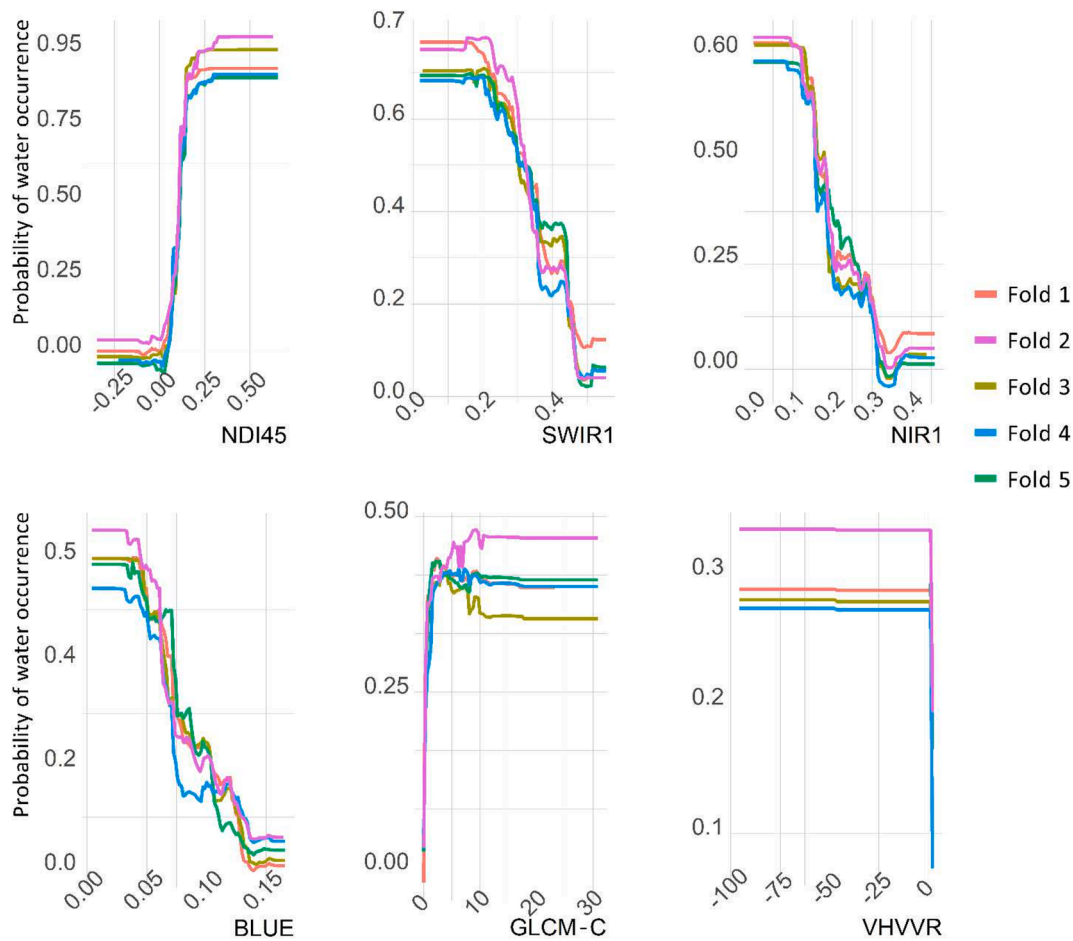
Fig. 3. Partial dependence plots of most important variables explaining surface water occurrence. For each variable, multiple curves are depicted, with each color representing a fold of the stratified RF cross-validations. Additional plots of the remaining variables can be found in Supplementary Materials (Figure SM2.5).
