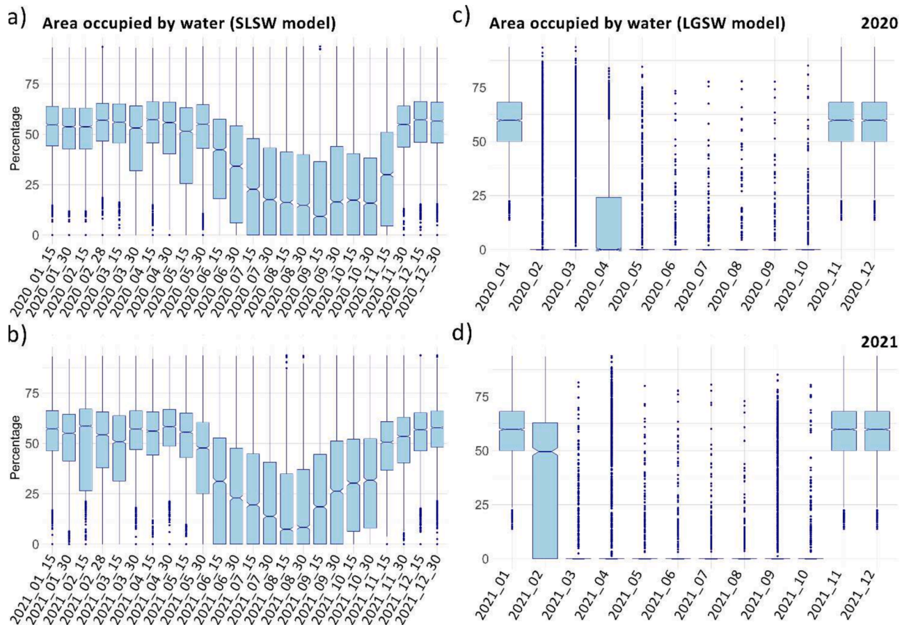
Fig. 4. Surface water extent, considering the three semiarid regions collectively. The time series represent the SLSW model for both 2020 (a) and 2021 (b), and the LGSW model for both 2020 (c) and 2021 (d), with a time interval of 15 days and 30 days, respectively. For each date, the range of values illustrates the water extent percentage within water bodies, with dots depicting the outliers.
