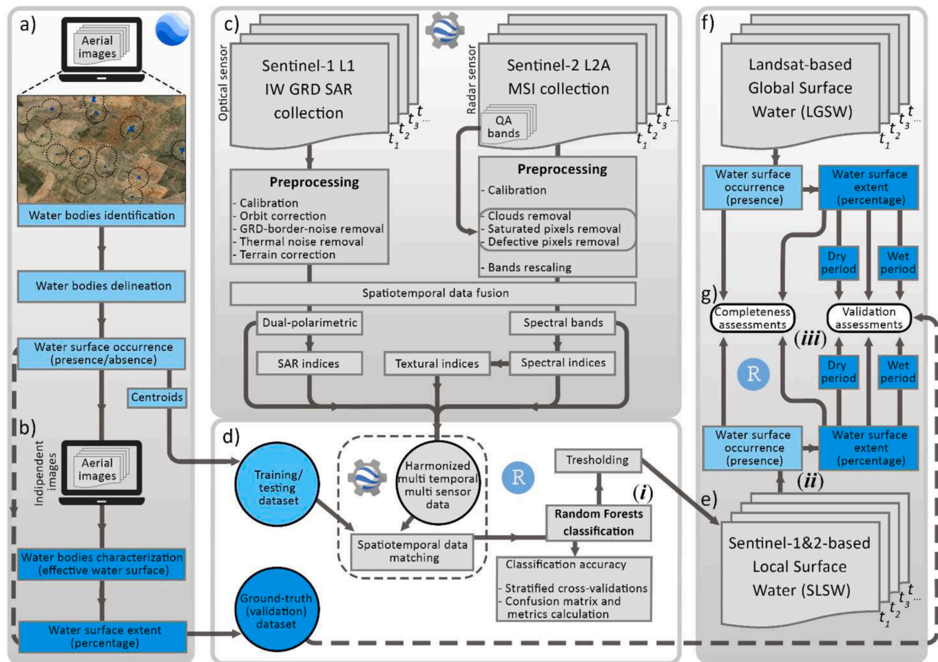
Fig. 2. Framework diagram depicts the analytical steps across four main panels, where arrows represent the operational progressions. The left panel illustrates how water bodies' datasets were prepared, namely surface water occurrence (a) and extent (b), whilst the central-upper panel (c) shows how satellite (Sentinel-1&2) image time series were pre-processed and how variables were calculated. The central-lower panel (d) indicates how data were compiled for subsequent analyses to respond to the first objective (i). The right panel depicts the second (ii) and third (iii) objectives, following the characterization of the SLSW time series (e) and the comparative assessment with the LGSW time series (f).
