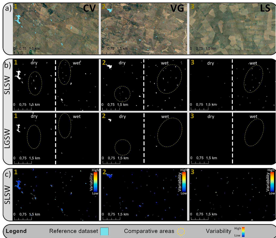
Fig. 6. Surface water distribution in the magnified areas (a), where numbers indicate their representative regions depicted in Fig. 1. The magnified areas were comparable concerning surface water occurrence predictions (in white) by SLSW (upper panels) and LGSW (middle panels) (b), jointly with SLSW-derived variability (lower panels) (c). Upper and middle panels were bisected by a vertical (white) dashed line, to represent dry (August) and wet conditions (January). Ellipses and circles are also depicted in magnified areas highlighting clustered water bodies, to emphasize prediction comparisons between SLSW and LGSW.
