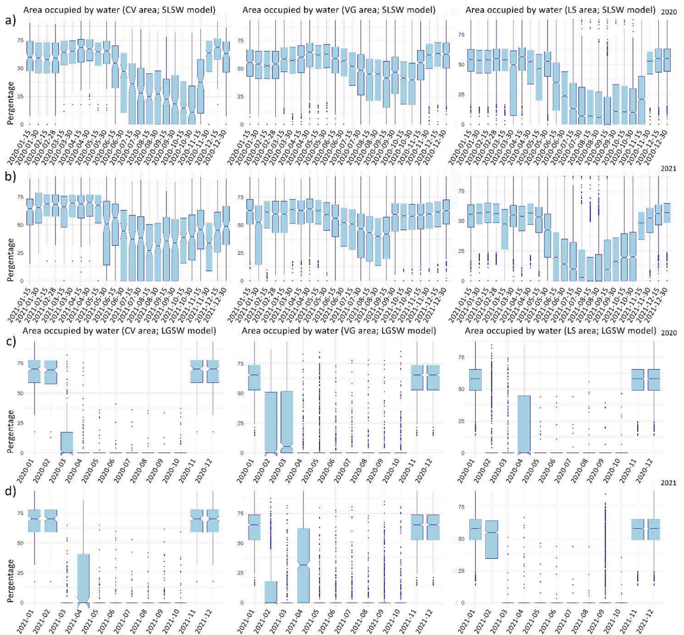
Fig. 5. Surface water extent, considering the three semiarid regions (CV, VG, and LS; Fig. 1) separately. The time series represent the SLSW model for both 2020 (a) and 2021 (b), and the LGSW model for both 2020 (c) and 2021 (d), with a time interval of 15 days and 30 days, respectively. For each date, the range of values illustrates the water extent percentage in water bodies, with dots depicting the outliers.
