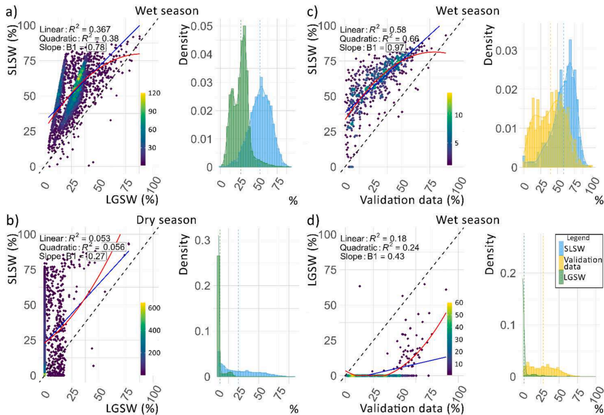
Fig. 7. Density scatterplots are depicted with the linear (blue line) and quadratic (red line) regressions between SLSW and LGSW models concerning surface water extent percentage under both wet (a) and dry conditions (b). Furthermore, independent comparisons of SLSW and LGSW models with the validation dataset are presented in separate panels (c and d). In all panels, each graph point is a representation of a distinct water body. Density plots are coupled with each regression, where dashed lines represent the median value of estimated surface water extent. (For interpretation of the references to color in this figure legend, the reader is referred to the web version of this article.)
