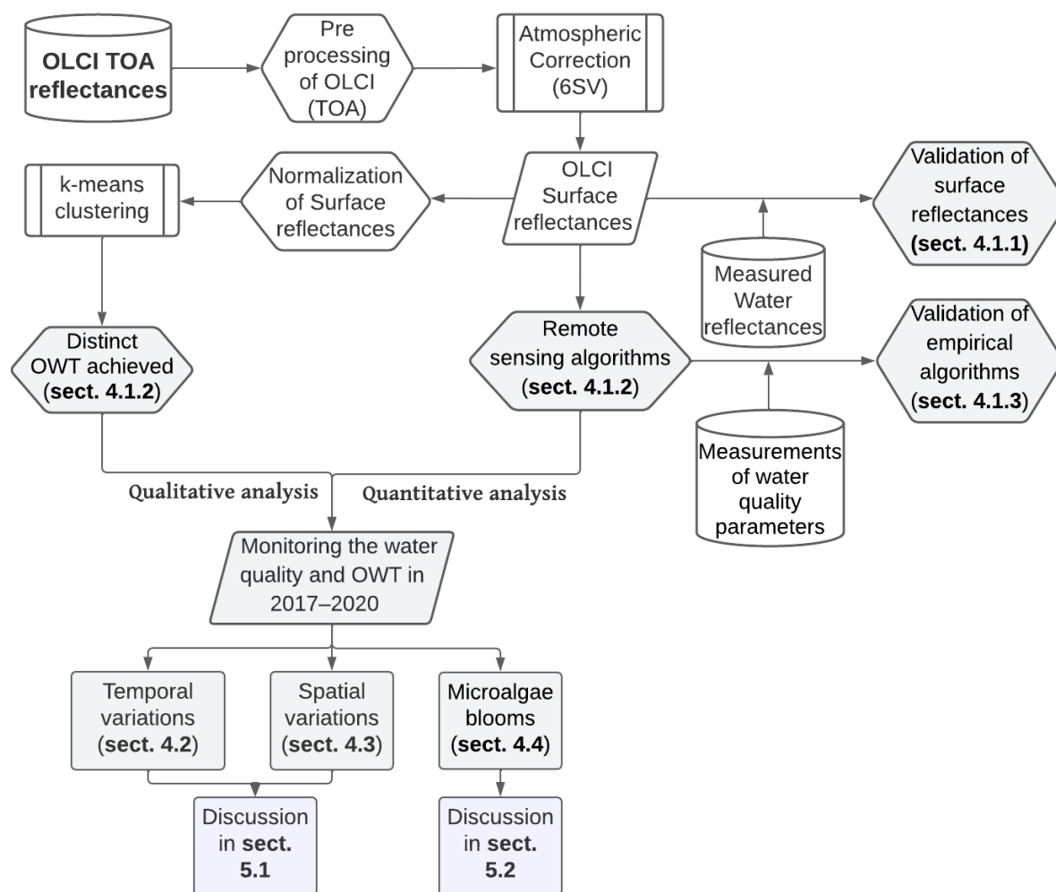
Figure 3. Flowchart showing the methodology using OLCI data and the main results (gray background) obtained in this work.
