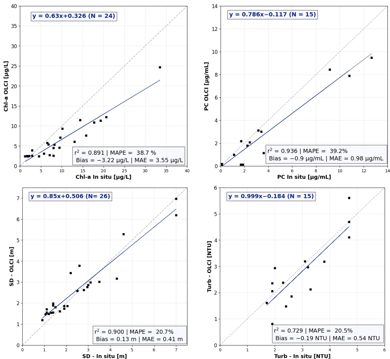
Figure 6. Scatter plot of predicted versus measurements/laboratory data (Chl-a and PC on the top panel; SD and Turb on the bottom panel).
