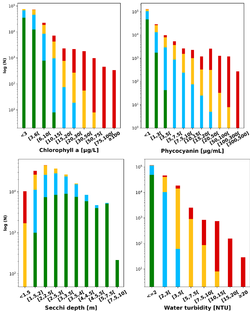
Figure 11. Number of pixels per OWT cluster and for each of the classes of water quality parameters. The figures above represent Chl-a concentrations (left) and PC concentrations (right). Below represent SD (left) and Turb (right). The green bars represent OWT1, in blue OWT2, in orange OWT3, and red is OWT4.
