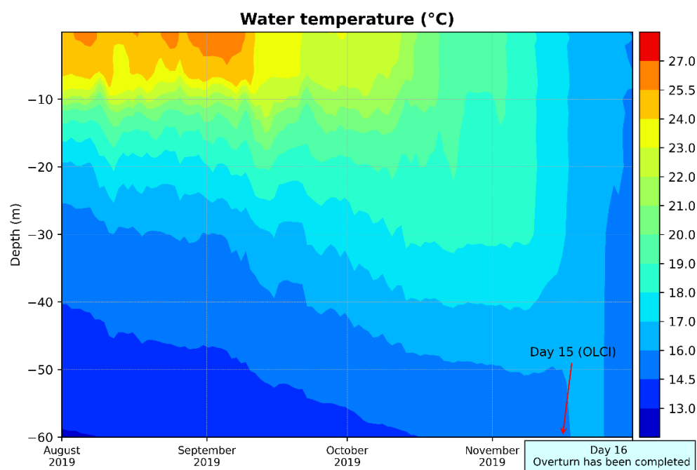
Figure 10. Temperature profile from August to November (2019).
