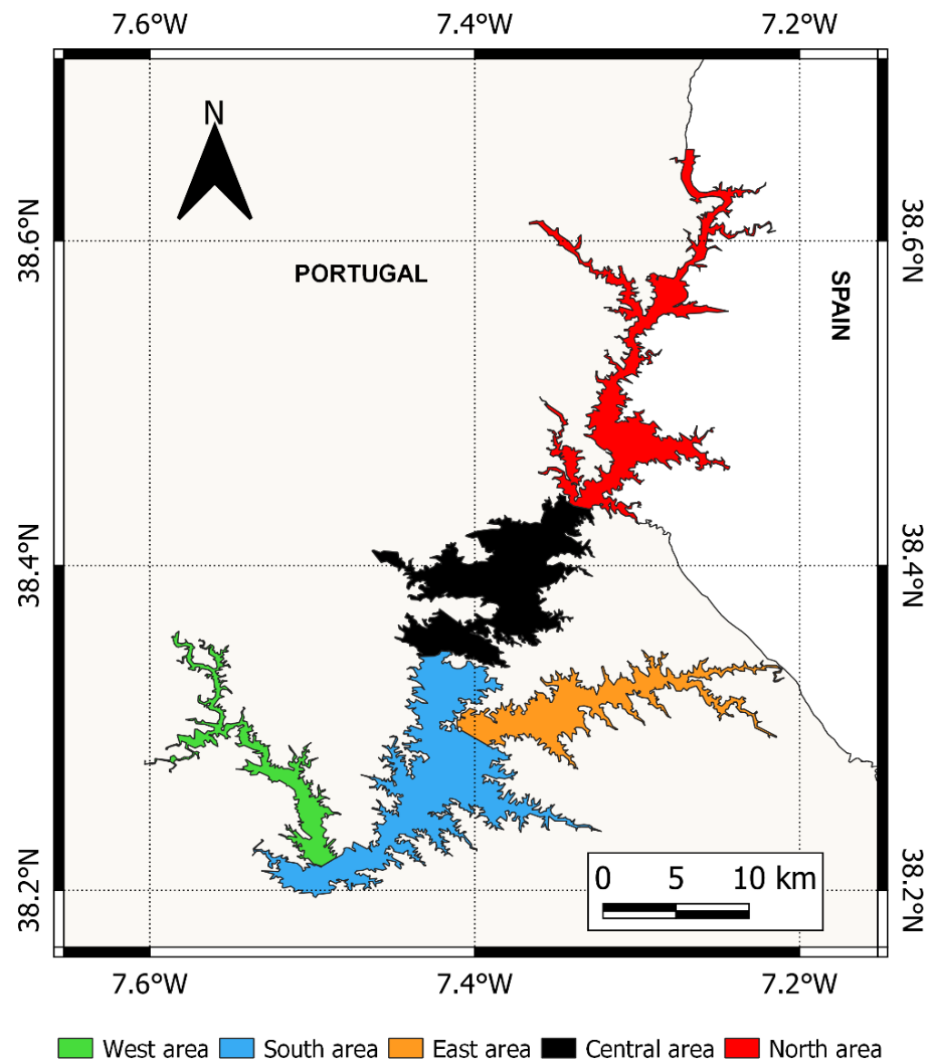
Figure 1. Alqueva reservoir divided into five areas for water quality analysis.
