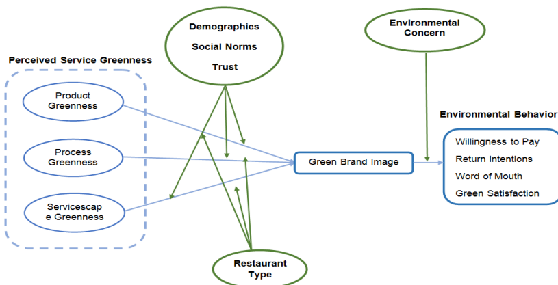
Figure 1. Proposed model
