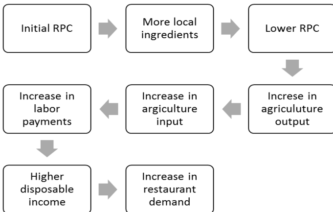
Figure 2. Proposed model
