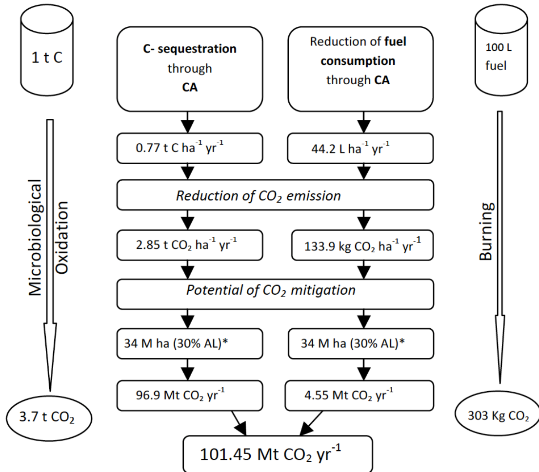
Figure 2. Estimation of the potential reduction CO 2 emissions through the application of Conservation Agriculture in Europe (EU-27). *When applied on 30% of total European Arable Land (AL), 113.4 Mha [41].
